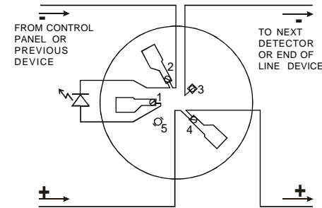
Figure 2a: Non-Resistor Base Wiring
